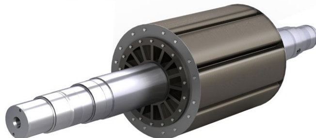
Rotor of the PM generator
